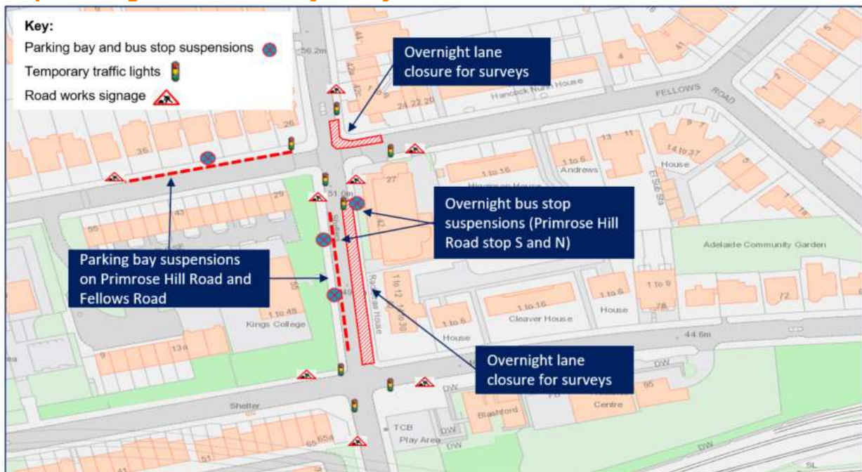
Map showing location of utility surveys on Primrose Hill Road and Fellows Road
